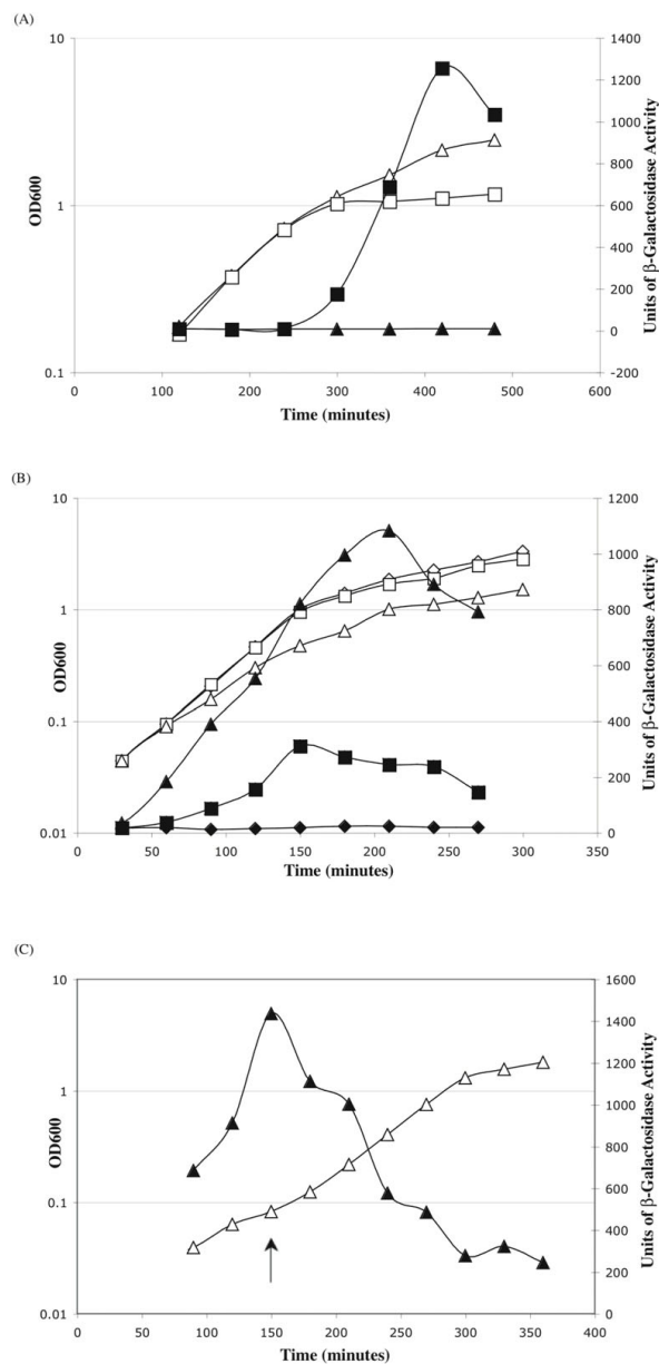
Figure 1 Response of the B. cereus lysK T-box regulatory element to reduced tRNA Lys charging. Growth is represented by open symbols and β-galactosidase activity by closed symbols. Representative expression profiles are presented. Growth is represented by open symbols and β-galactosidase activity by closed symbols. (A) Growth and β-galactosidase accumulation in strain NF33 ( P_{lysK(T\ box)} lacZ ) in minimal media. Strain NF33 was grown in minimal medium containing 100 μg/ml lysine (triangles) and 20 μg/ml lysine (squares). (B) Growth and β-galactosidase accumulation in strain BCJ367 ( P_{lysK\ Tbox} lacZ\ P_{spac\ lysS\ pMap65} ) in LB containing varying IPTG concentrations: 1 mM IPTG (diamonds); 250 μM IPTG (squares) and 100 μM IPTG (triangles). (C) Growth and β-galactosidase activity of strain BCJ367 in LB containing 100 μM IPTG. The IPTG concentration was increased to 1 mM at 150 minutes, indicated by the arrow.
